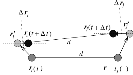
Figure 15.4 Coordinate resetting to realize a bond length constraint.
