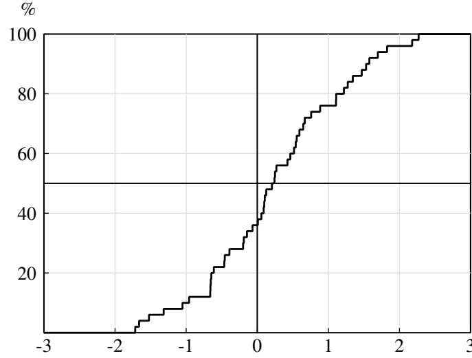
Figure 19.5 Cumulative distribution of 50 samples taken from a normal distribution.
