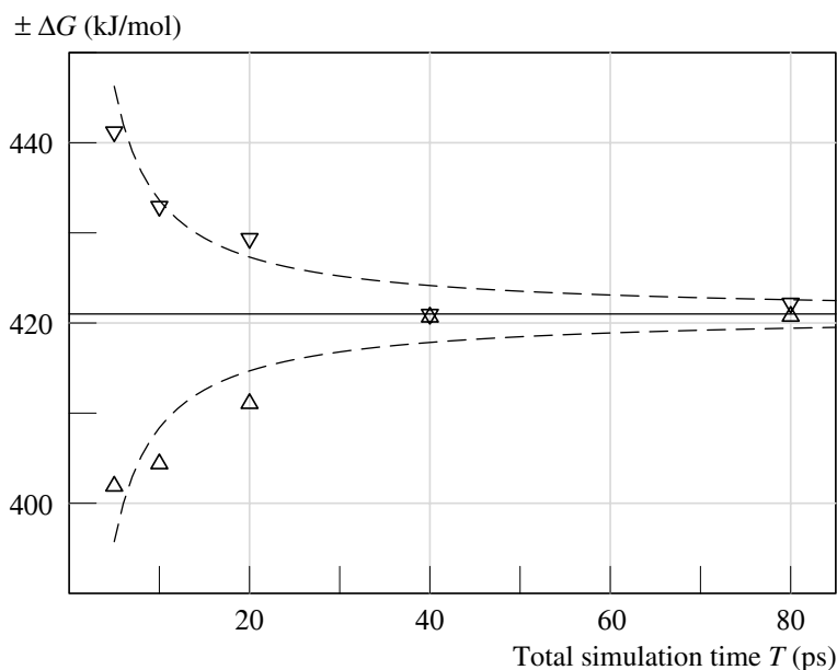
Figure 7.2 Free energy change resulting from transforming a model neon atom into a sodium ion in a bath of 216 water molecules, by linearly increasing the charge on the atom in a total simulation time T . Upward triangles are for growth from Ne to \text{Na}^+ , yielding a negative \Delta G ; downward triangles are for the opposite change. Dashed curves are predictions from the theory of Wood (1991) assuming a relaxation time for the ensemble of 0.15 ps. Data are from Straatsma and Berendsen (1988).
