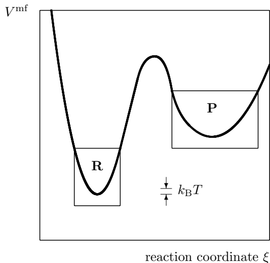
Figure 7.3 Potential of mean force in one “reaction coordinate” \xi . There are two regions of configurational space ( R and P ) that can be designated as confining a thermodynamic state.
