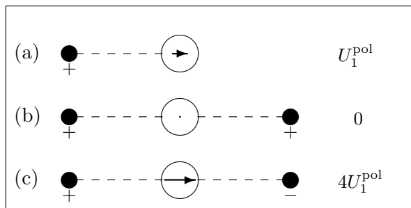
Figure 6.8 The non-additivity of polarization energies. (a) a single charge that polarizes a neutral particle causes an induced dipole and a (negative) polarization energy; (b) The fields of two equal, but oppositely placed, charges compensate each other; there is no polarization energy; (c) When the fields add up, the polarization energy due to two charges is four times the polarization energy due to one charge.
