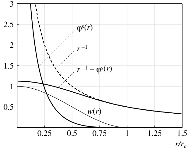
Figure 13.7 Functions for the cubic spread function: w(r) is proportional to the spread function; the potential functions are as in Fig. 13.6, but scaled by 2 to make them comparable.
