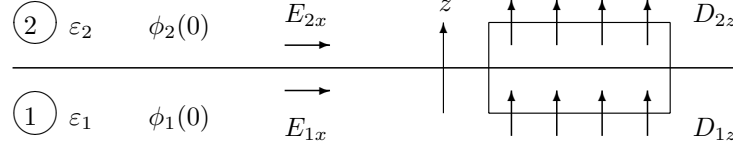
Figure 13.1 Boundary conditions on a planar discontinuity: potential \phi , tangential electric field E_x and perpendicular displacement D_z are continuous.
