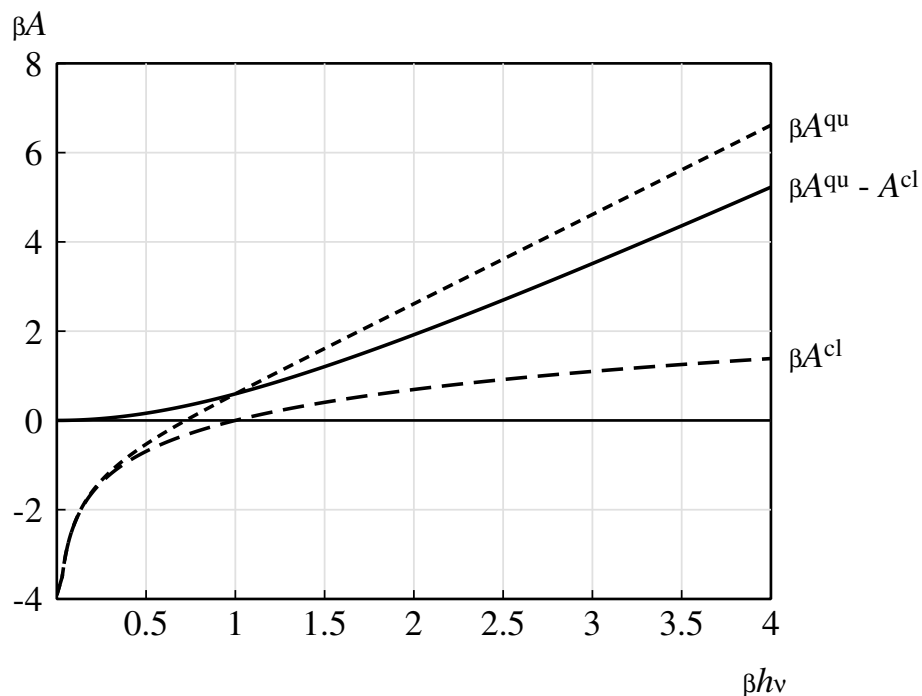
Figure 7.4 Helmholtz free energies divided by k_B T for a single harmonic oscillator, as a function of h\nu/k_B T , for both classical and quantum-mechanical statistics. The drawn line gives the quantum correction to a classical free energy.
