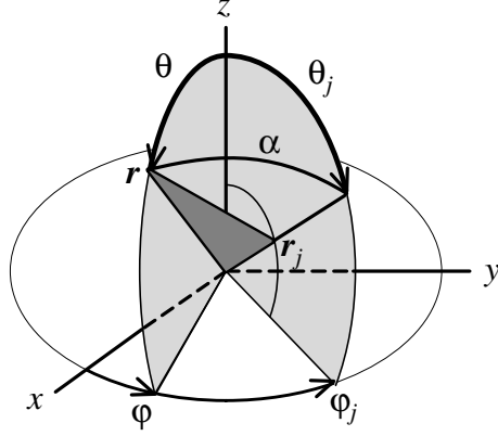
Figure 13.4 The source is at \mathbf{r}_j = (r_j, \theta_j, \phi_j) and the potential is determined at \mathbf{r} = (r, \theta, \phi) . The angle between these two vectors is \alpha .
