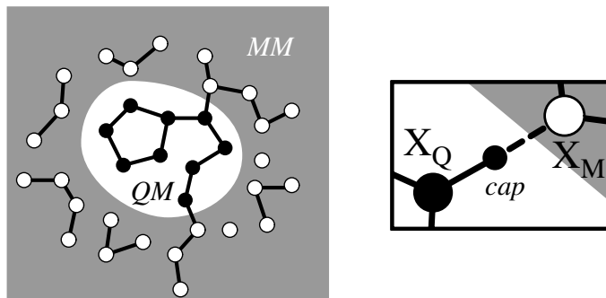
Figure 6.11 A quantum mechanical fragment embedded in a molecular mechanics environment. Covalent bonds that cross the QM-MM boundary are replaced by a cap atom in the QM part.
