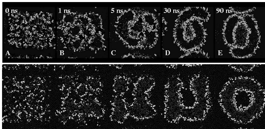
Figure 8.1 Two simulations of the spontaneous formation of a lipid bilayer vesicle. Upper panel: atomic detail molecular dynamics; lower panel: coarse-grained super-atom dynamics simulation (Courtesy of S.-J. Marrink and A. H. de Vries, University of Groningen; reproduced by permission from J. Comput. Chem. (van der Spoel et al. , 2005))
