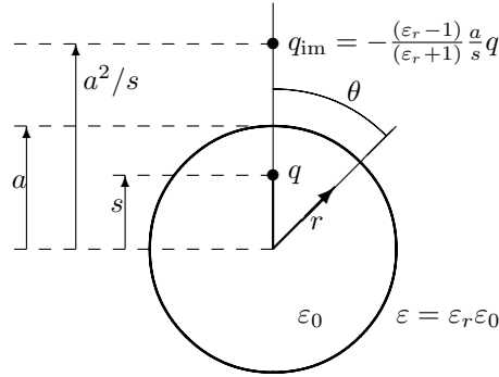
Figure 13.2 A source charge q in a vacuum sphere, embedded in a dielectric medium, produces a reaction potential that is well approximated by the potential of an image charge q_{\text{im}} situated outside the sphere.
